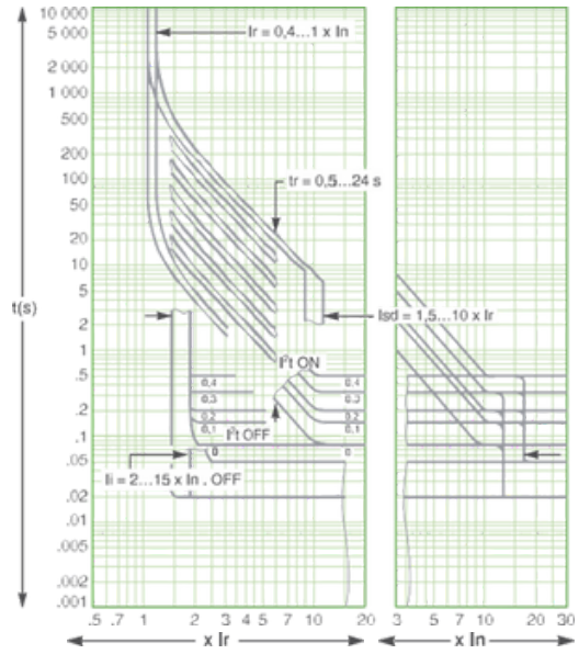
Micrologic Universal Planck V800
