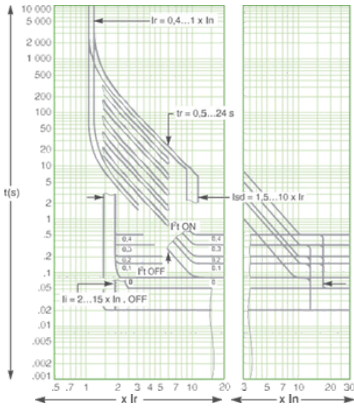
Micrologic Universal Planck V800
